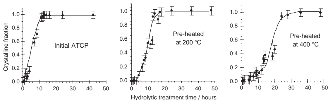
Fig. 5. Evolution of the crystalline fraction for the lyophilized samples obtained after the hydrolytic treatment at 25 °C in deionized water for different times of the lyophilized and pre-heated ATCPs.
