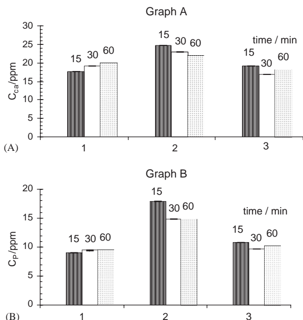
Fig. 7. Variation of the ionic concentrations of calcium (Graph A) and phosphate (Graph B) in hydrolysis solutions obtained after 15, 30 and 60 min of the immersion at 25 °C in deionized water of ATCPs (1) lyophilized, (2) pre-heated at 200 °C and (3) pre-heated at 400 °C.
