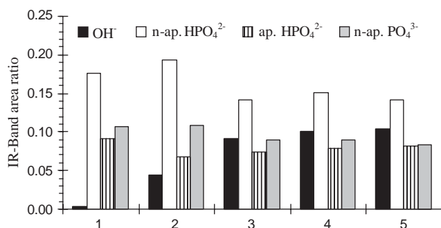
Fig. 4. Band area ratio of OH - ions, non-apatitic (nap.: labile) and apatitic (ap.) HPO 4 2- and non-apatitic PO 4 3- groups of the lyophilized ATCP after apatitic conversion with hydrolytic treatment times (1) 12 h 30 min, (2) 18 h, (3) 24 h, (4) 48 h and, (5) 96 h.
