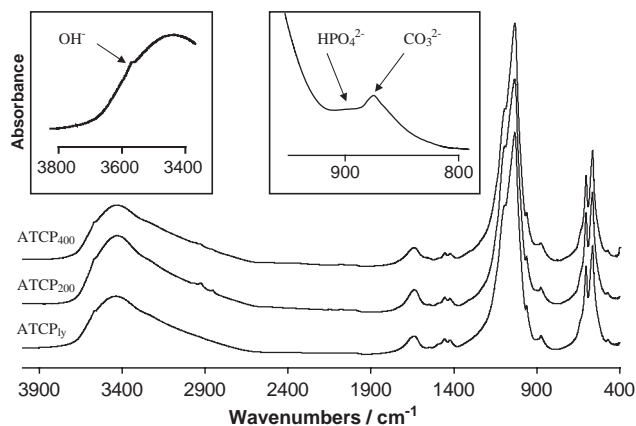
The spectra are very similar. The enlargements show the OH - stretching vibration at 3570 cm -1 and the HPO 4 2- (broad band) and carbonate bands (small narrow band) at 870 cm -1 .
