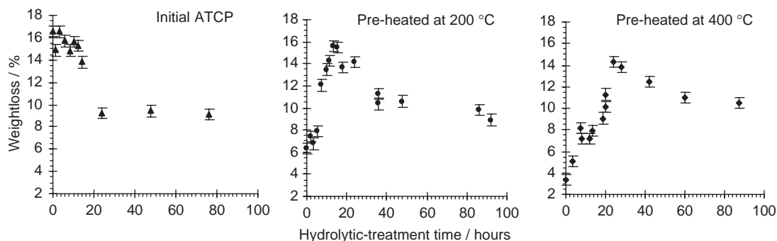
Fig. 6. Evolution of the weight TG-loss, between 50 and 500 °C, of the lyophilized products obtained after the hydrolytic treatments at 25 °C in deionized water for different times of lyophilized and pre-heated ATCPs.
