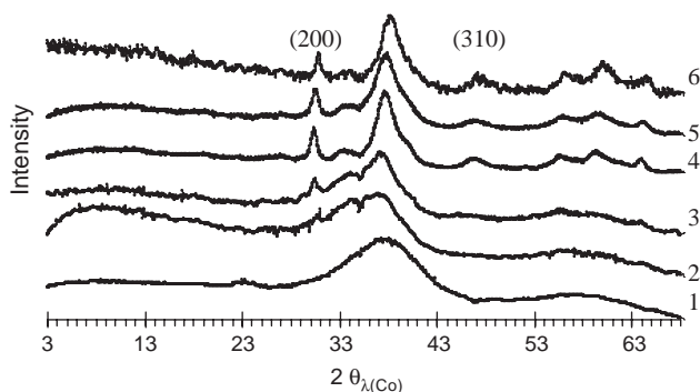
Fig. 2. Evolution of XRD diagrams during the isothermal hydrolytic treatment at 25 °C of the ATCP pre-heated at 200 °C: (1) 0, (2) 4, (3) 10, (4) 14, (5) 20 and, (6) 48 h.
