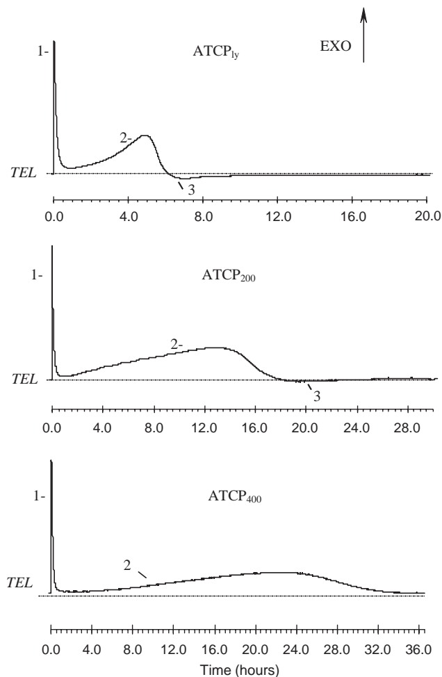
Fig. 1. Isothermal microcalorimetric curves at 25 °C for the hydrolytic treatments of the lyophilized and pre-heated ATCPs in deionized water: (1) first peak, (2) second peak, (3) endothermic peak and, TEL: Representation of the Thermal Equilibrium Line.
